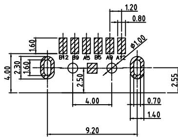
RECOMMENDED P. C. B LAYOUT TOP VIEW (TOLRANCE: ±0.05)
